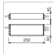
LED OSRAM OT power supply zasilacz LED OSRAM OT 240W/220-240/24V P
