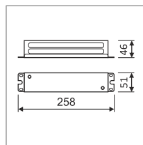
LED OSRAM OT power supply zasilacz LED OSRAM OT 120W/220-240/24V E
