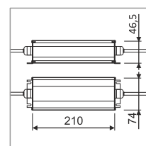
LED power supply zasilacz LED 12V/150W; 200-240V; IP68
