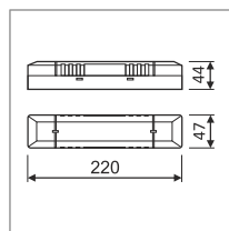
LED OSRAM OT power supply zasilacz LED OSRAM OT 75W/220-240/24V
