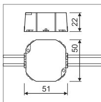
LED OSRAM OT power supply zasilacz LED OSRAM OT 6W/200-240/24V CE
