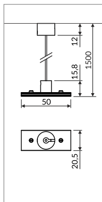
sling for LED mounting 1500 zawiesie do uchwytu LED 1500
