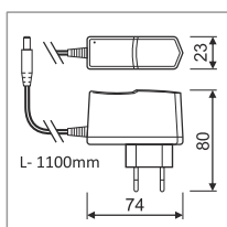
LED power supply AC adapter zasilacz LED wtyczkowy 12V/12W; 100-240V
