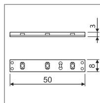
LED strip 3528 (B) taśma LED 3528 (B) 12V; 4,8W/m; 60P/m; IP65
