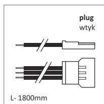
LED cable with plug przewód LED 1xW 3x0,22; L-1800; MIKRO3
