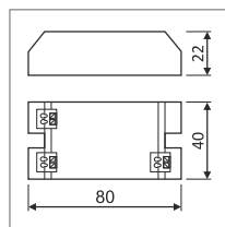
LED OSRAM OT power supply zasilacz LED OSRAM OT 8W/200-240/24V
