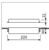
LED OSRAM OT power supply zasilacz LED OSRAM OT 30W/220-240/24V P
