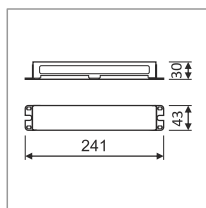
LED OSRAM OT power supply zasilacz LED OSRAM OT 75W/220-240/24V E
