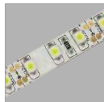
LED strip 3528 (B) taśma LED 3528 (B) 12V; 9,6W/m; 120P/m; IP65
