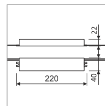
LED OSRAM OT power supply zasilacz LED OSRAM OT 50W/220-240/24V P
