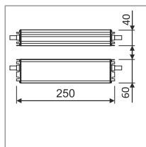
LED OSRAM OT power supply zasilacz LED OSRAM OT 120W/220-240/24V P
