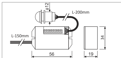
movement sensor YCB1050 czujnik ruchu YCB1050 230V/800W
