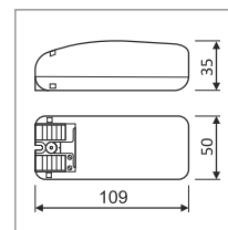
LED OSRAM OT power supply zasilacz LED OSRAM OT 20W/220-240/24V
