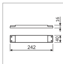
LED OSRAM OT power supply zasilacz LED OSRAM OT 50W/220-240/24V
